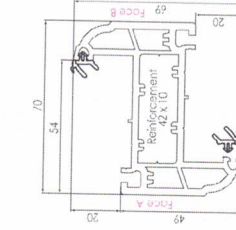
546675 576675 (FOILED) SLIM SCULPTURED TRANSOM/MULLION 'T' 69MM
