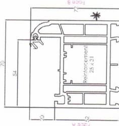
546435 586435 (FOILED) CASEMENT UNIVERSAL SCULPTURED OUTER FRAME 72MM (5 CHAMBERS)
