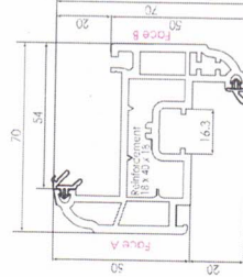
546695 576695 (FOILED) SCULPTURED TILT/TURN SASH 70MM
