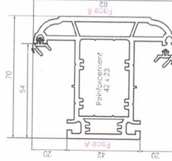
546745 576745 (FOILED) LARGE SCULPTURED TRANSOM/MULLION 'T' 82MM
