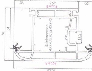
546725 576725 (FOILED) SCULPTURED DOOR 'T' SASH 105.5MM
