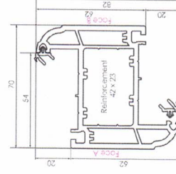
546755 576755 (FOILED) LARGE SCULPTURED TRANSOM/MULLION 'T' 82MM
