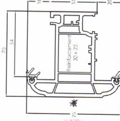
546455 576455 (FOILED) CASEMENT SCULPTURED 'T' SASH 75MM (5 CHAMBER)
